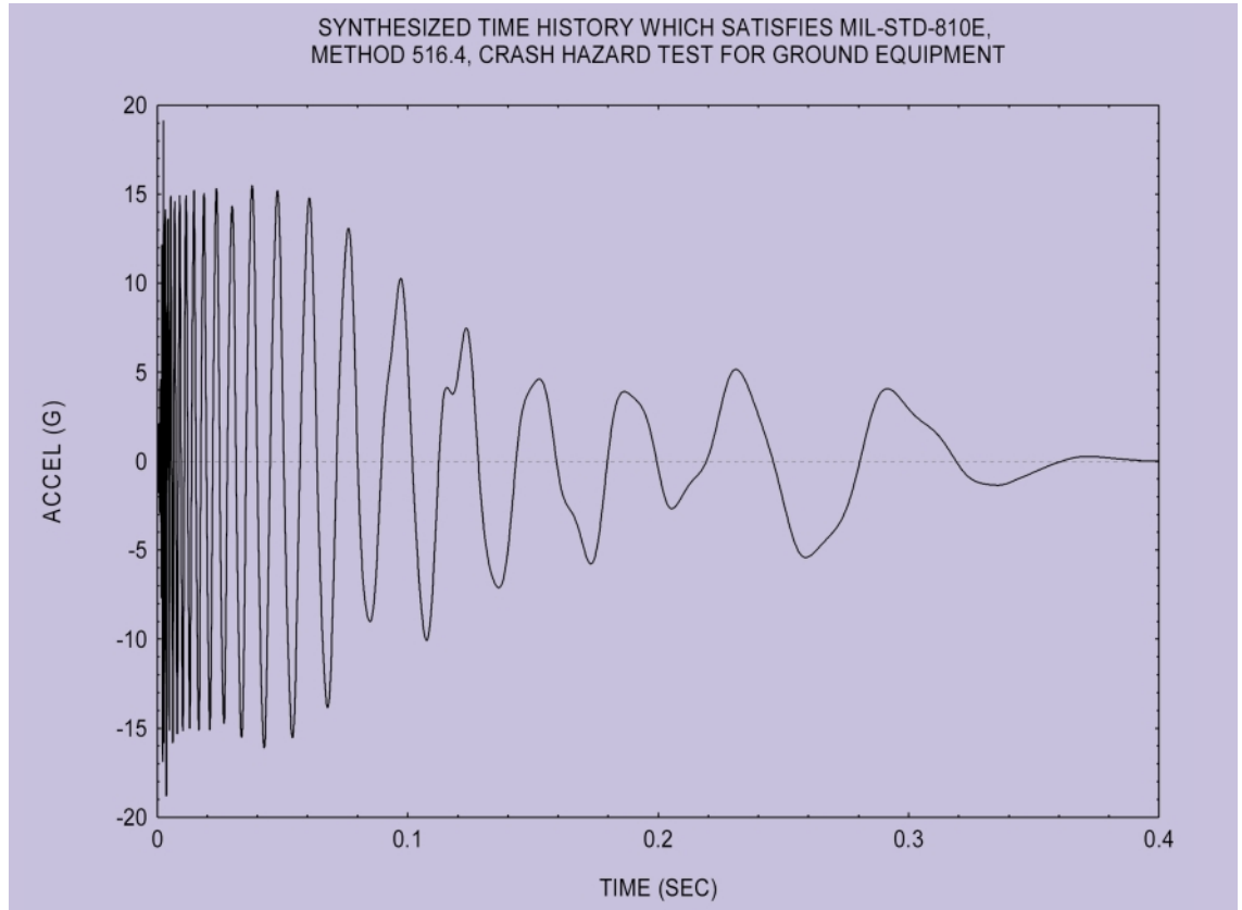
Figure 6. Synthesized Base Input Time History
