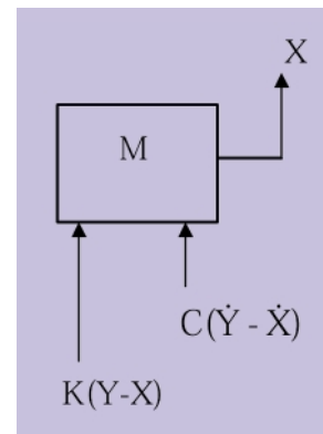
Figure 4. Free-body Diagram
