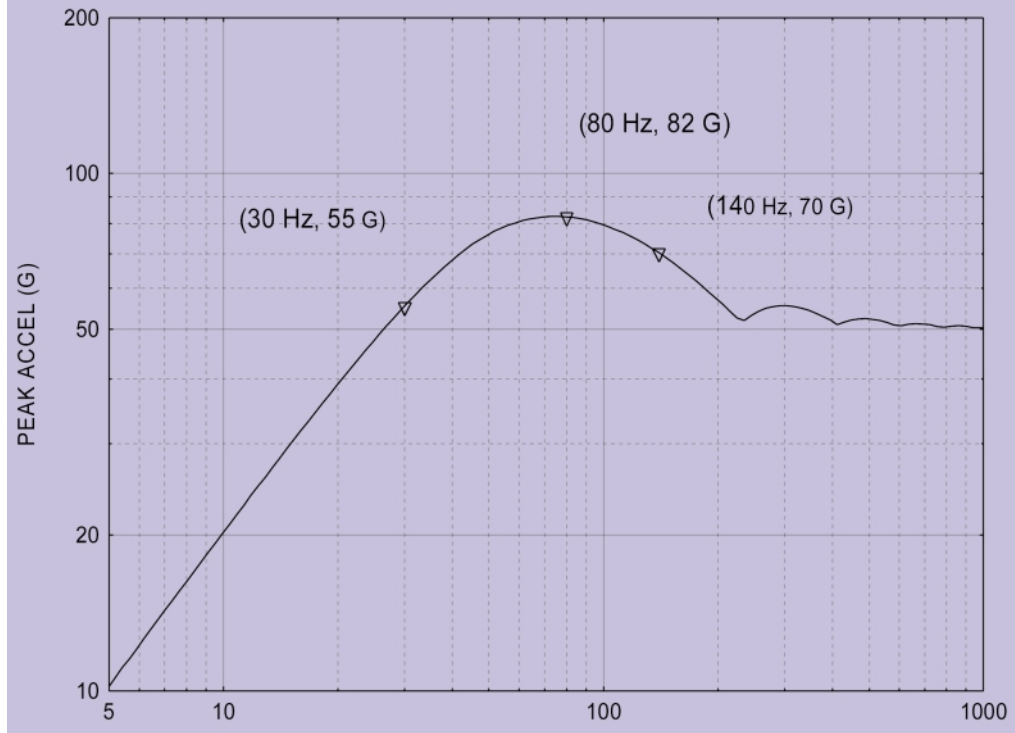
Figure 3. Corresponding Shock Response Spectrum
