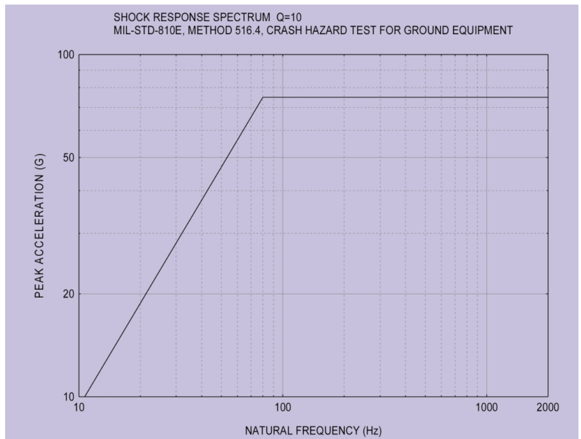
Figure 5. Shock Response Specification
