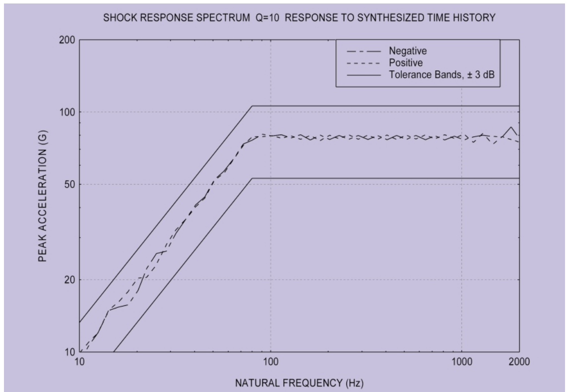
Figure 7. Shock Response Spectrum from Synthesized Base Input Time History
