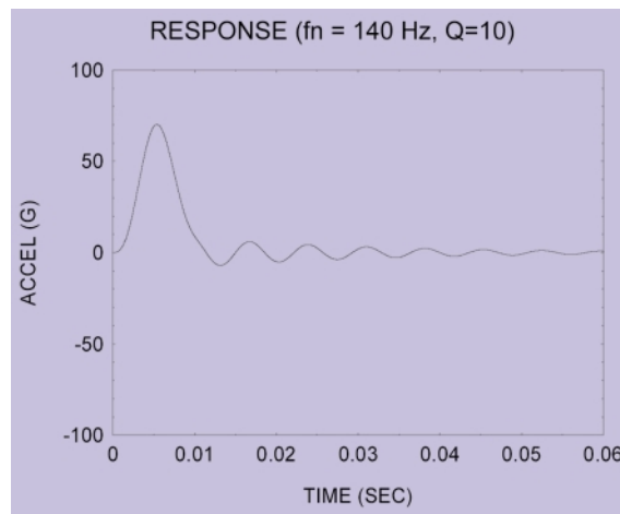
Figure 2. SDOF Response to Half-sine Base Input.
