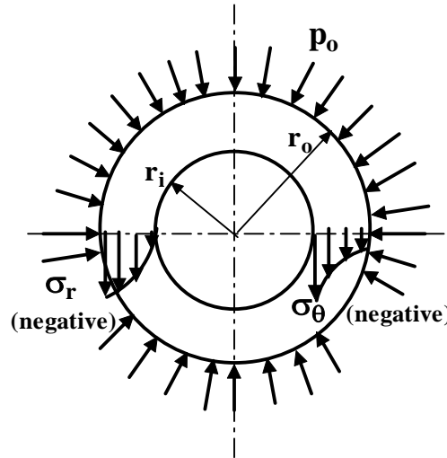
9.2.1.4F- Distribution of radial and circumferential stresses within the cylinder wall when only external pressure acts.
