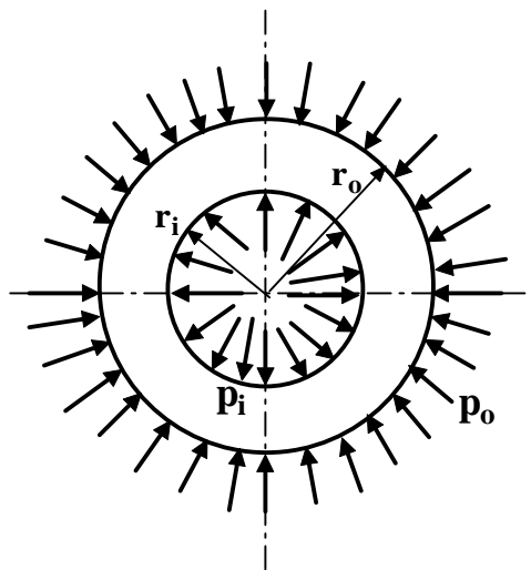
9.2.1.2F- A thick cylinder with both external and internal pressure.
