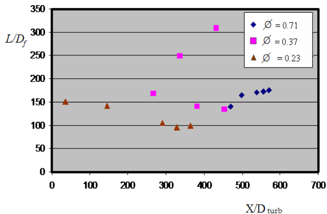
Fig. 9 Dimensionless flame height to extinguishment distance
