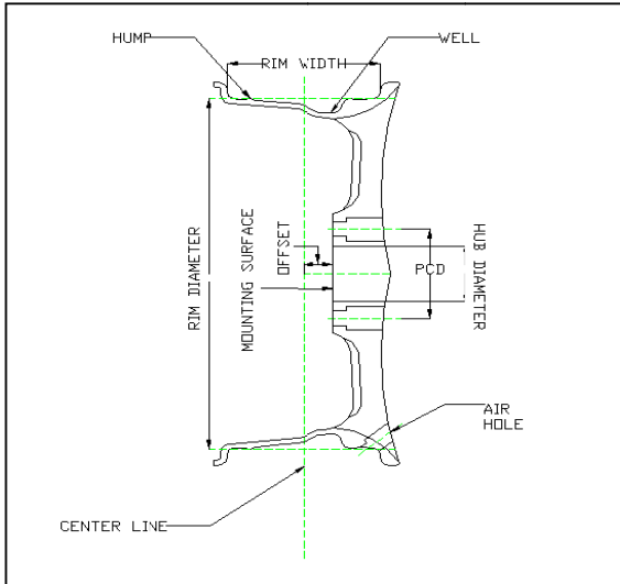
Figure 1. 2D Diagram of aluminum wheel
