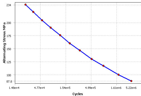
Figure 5 . Alternating Stress vs Cycle
