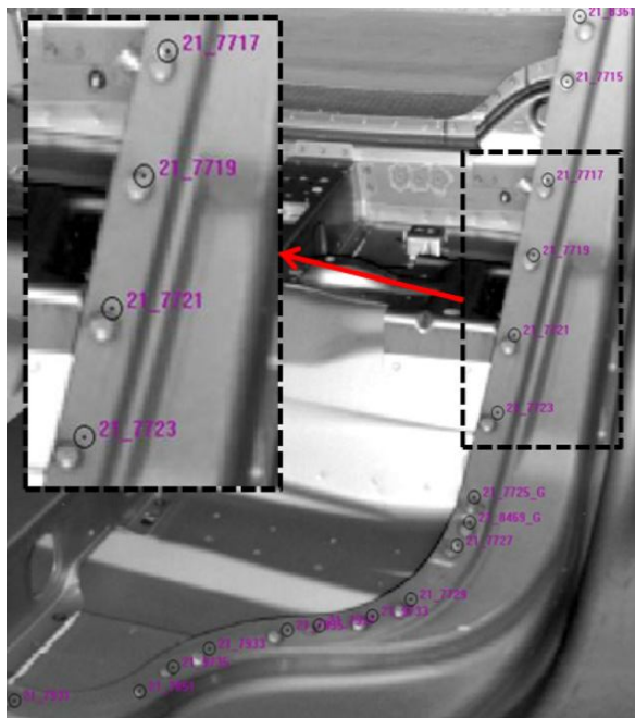
Fig. 4. The actual spot weld position compared to nominal spot weld position (indicated with black circles) [1].
