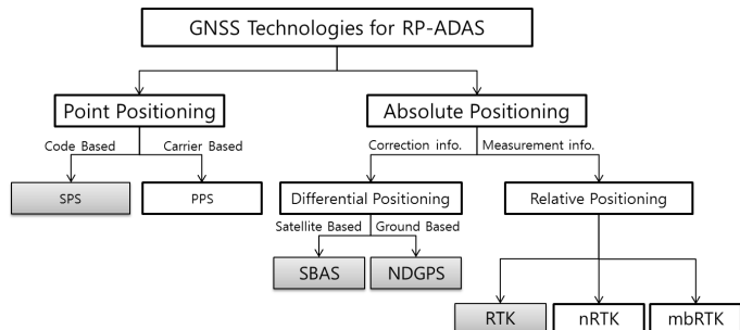
Fig. 5 GNSS Technology
