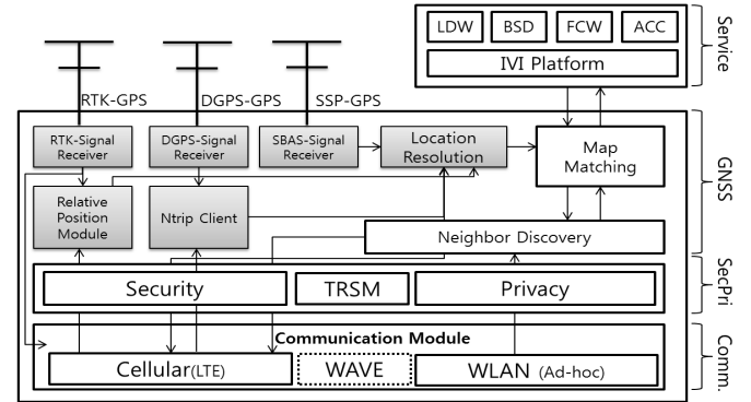
Fig. 3 RP-ADAS modules and Components
