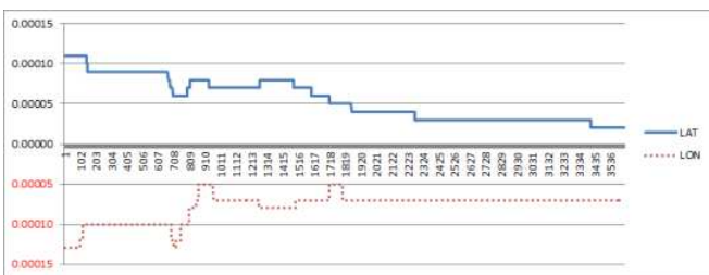
Fig. 11 Accuracy of DGPS receiver
