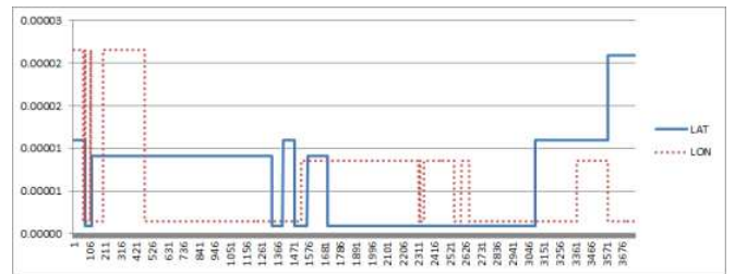
Fig. 13 Precision of SBAS receiver
