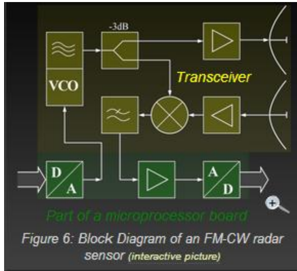
Figure 6: Block Diagram of an FM-CW radar sensor (interactive picture)
