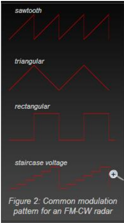
Figure 2: Common modulation pattern for an FM-CW radar
