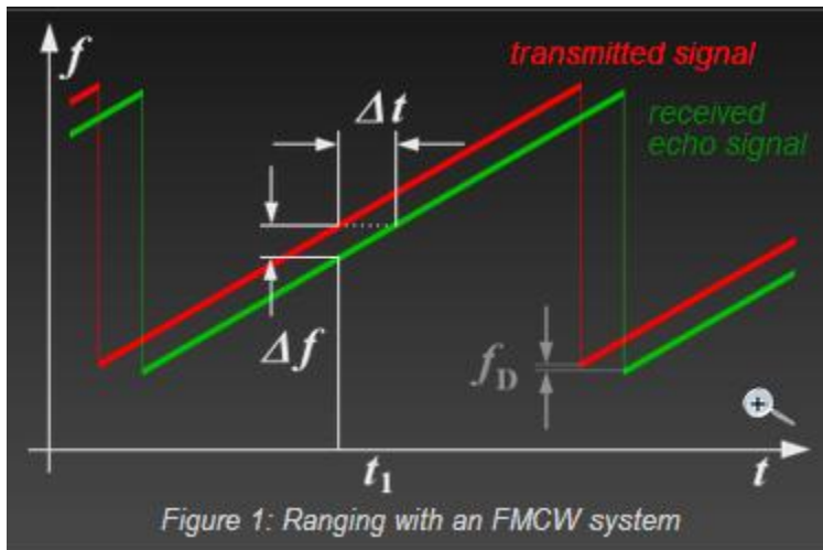
Figure 1: Ranging with an FMCW system
