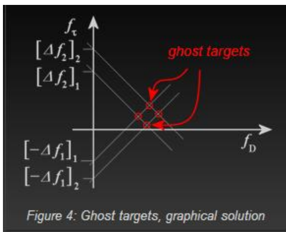
Figure 4: Ghost targets, graphical solution
