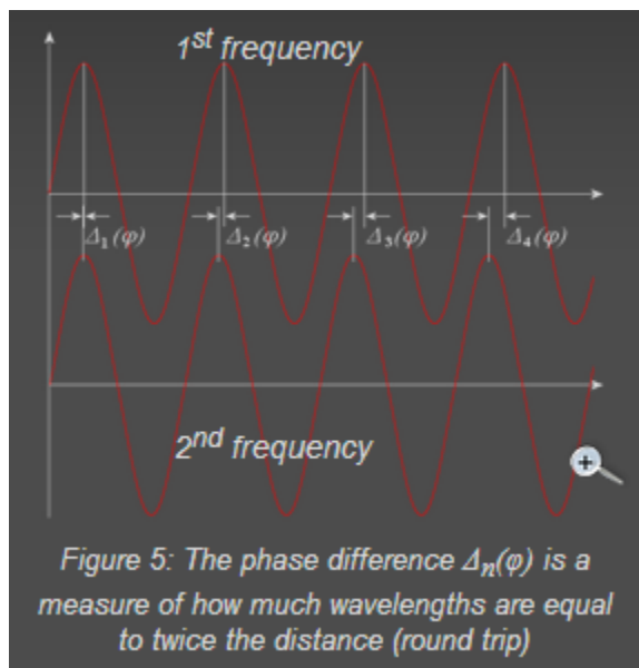
Figure 5: The phase difference \Delta_n(\varphi) is a measure of how much wavelengths are equal to twice the distance (round trip)
