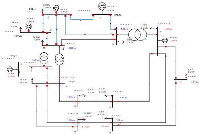
Fig. 2 IEEE 14 bus test power system configuration scheme
