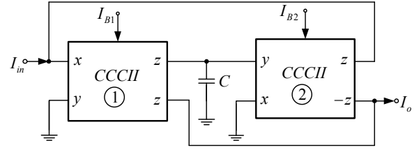
Fig. 3 Proposed current-mode first-order allpass filter
