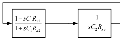
Fig. 7 Block diagram for quadrature oscillator
