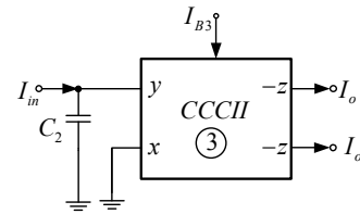
Fig. 8 Current-mode inverting lossless integrator based on CCCII
