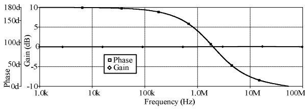
Fig. 4 Gain and phase responses of the proposed allpass filter
