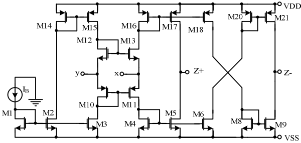
Fig. 2 Schematic of the CMOS CCCII
