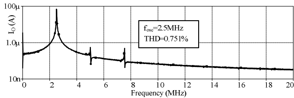
Fig. 11 The output spectrum of the oscillator
