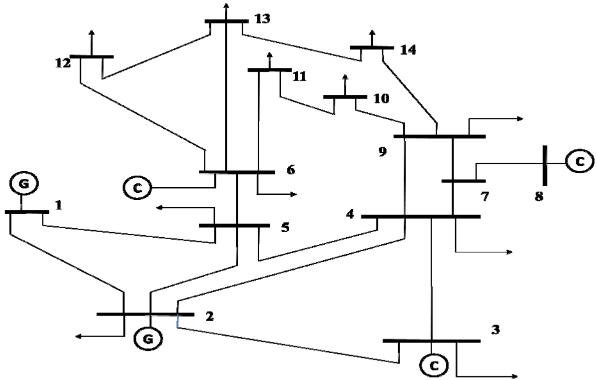
Fig 5. :IEEE 14 bus system
