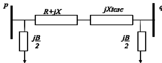
Fig 2. TCSC model with series reactance
