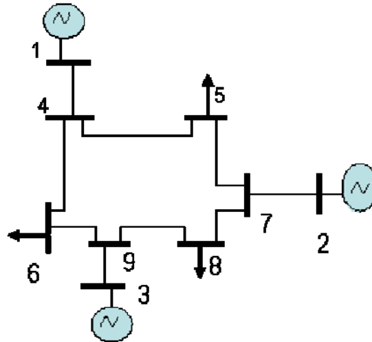
Fig. 4. 9-bus test System.
