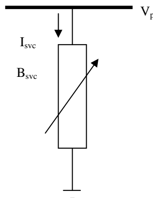
Fig 1. Variable shunt susceptance
