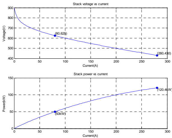
Fig. 3 The dynamic behavior of a PEMFC
