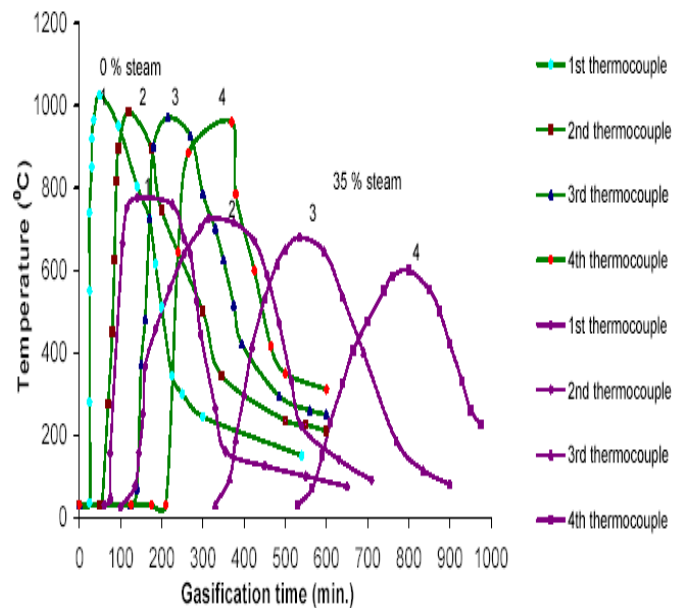
Fig. 5 Graphs ENVIRONMENTAL MERITS OF UCG
