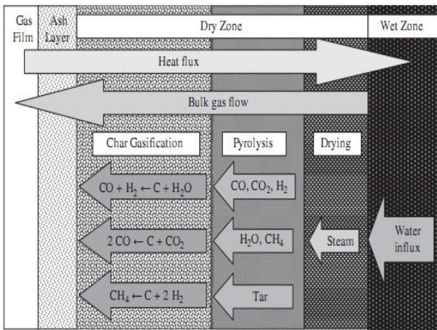
Fig:1(Zones and By-Products Of Coal Gasification)
