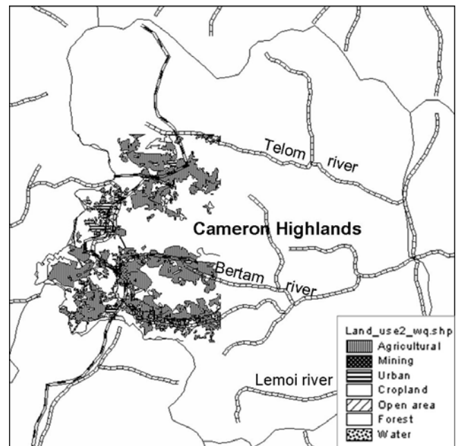
Fig. 1 Land uses and important rivers in Cameron Highland
