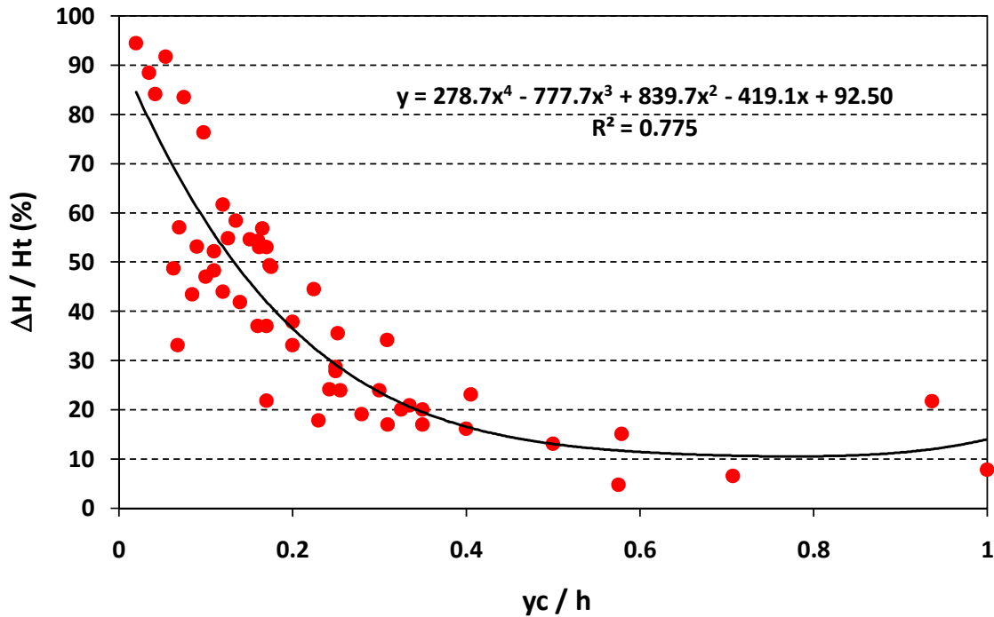
Fig. 6 Relation between \Delta H / H_t vs. y_c/h in vertical drop for all data (present study; Moore [3]; Chamani and Rajaratnam [7] and Rand [6])
