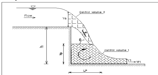
Fig. 1 Characteristics of flow over a vertical drop
