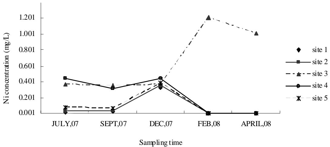
Fig. 9 C. Seasonal variations in Ni concentration in different month
