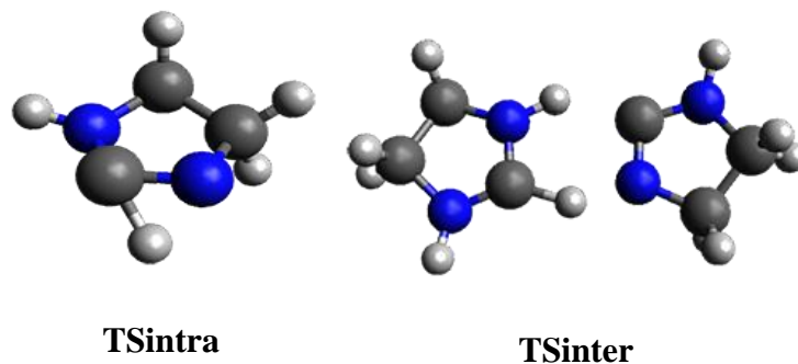
Figure 1. M06-2X/6-31+G(d,p) optimized transition states for Reactions 1 and 2.
