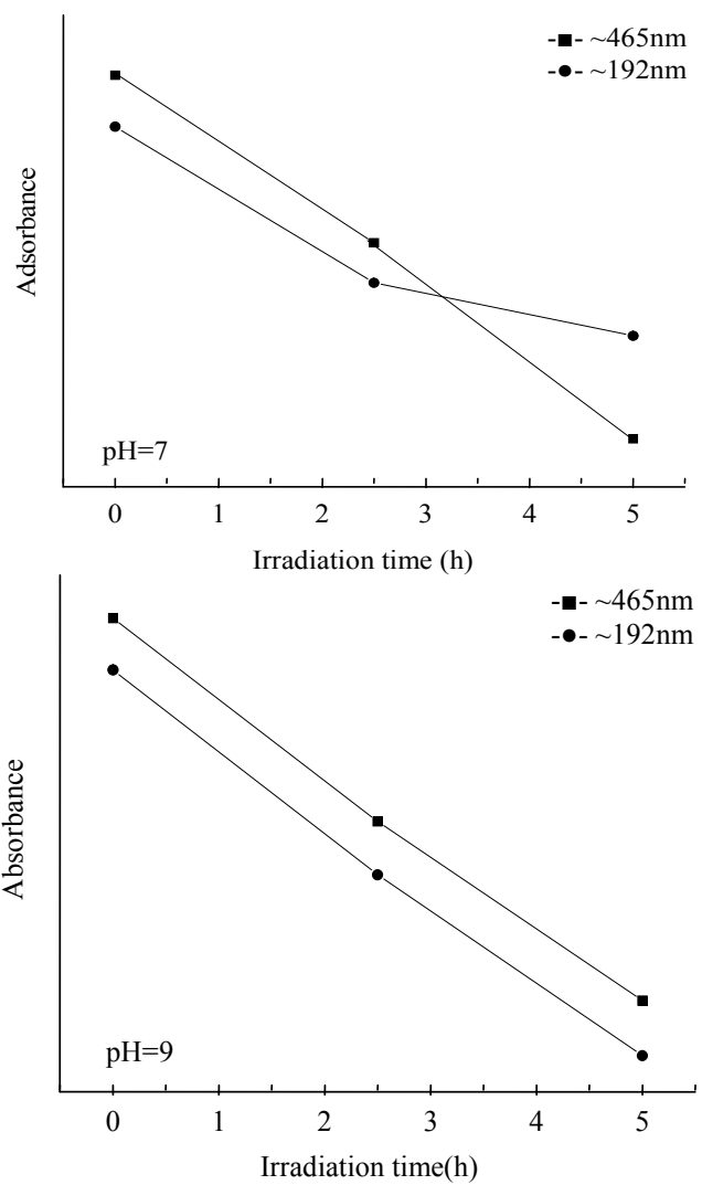
Fig. 3. Absorbance variations of methyl orange solution with irradiation time
