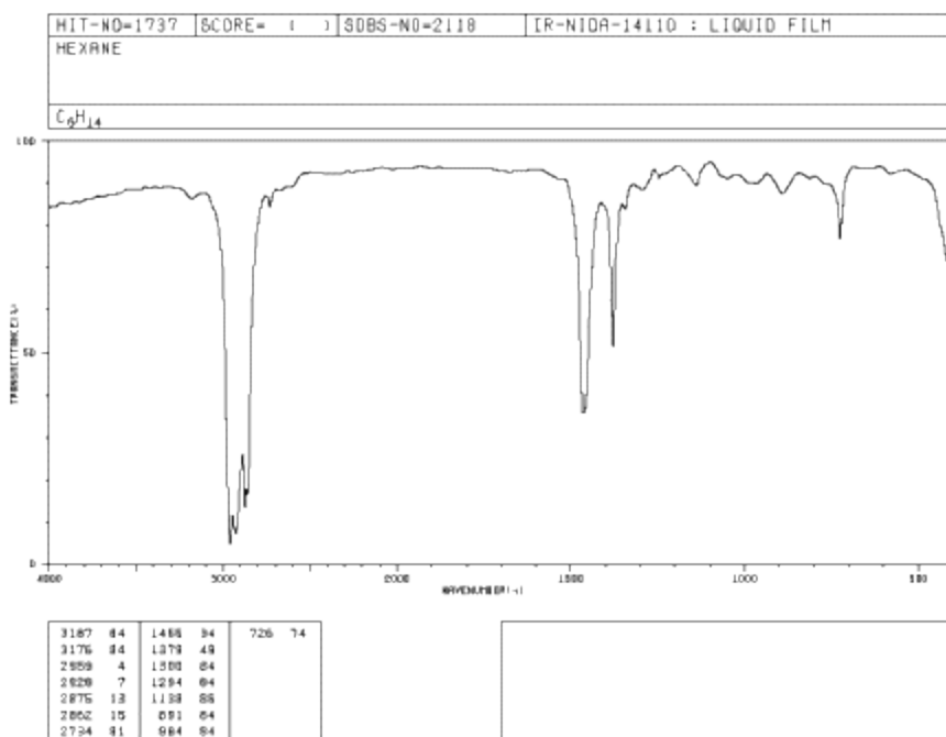
Figure IR2.1. IR spectrum of hexane.
