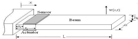
Figure 1 Cantilever Smart Sensor [1]
