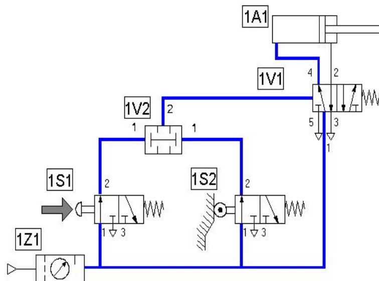
Figure 5.7 Two Pressure Valve
