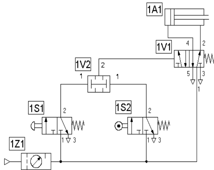
Figure 5.6 and Gate Combination
