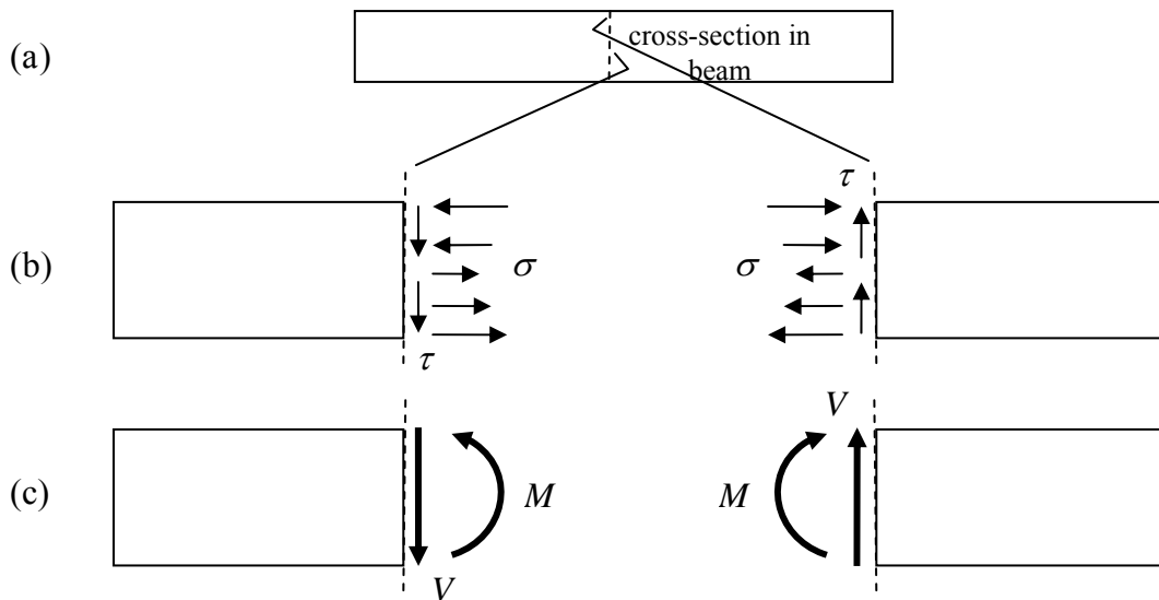
Figure 7.4.4: stresses and moments acting over a cross-section of a beam
