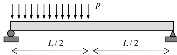
Figure 7.4.32: a simply supported beam subjected to a uniformly distributed load over half its length
