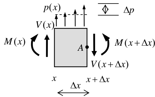
Figure 7.4.18: forces and moments acting on a small element of beam
