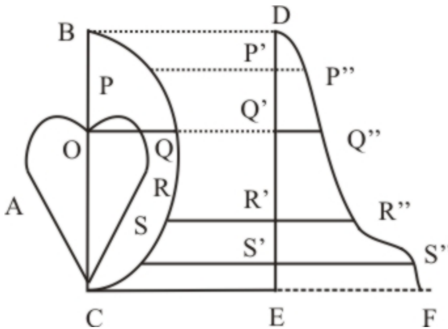
Fig. 8 Rousseau Diagram
