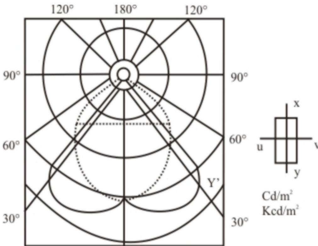
Fig.7 A typical Polar Luminance distribution diagram
