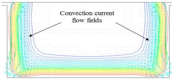
Fig. 12 Convective flow fields in 1 fin partition of Fin type configuration at 3600 seconds
