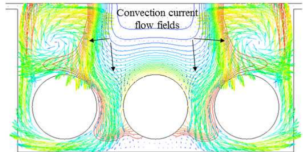
Fig. 5 Convective flow fields in 1 fin partition of fin-spiral filler configurations at 5400 seconds
