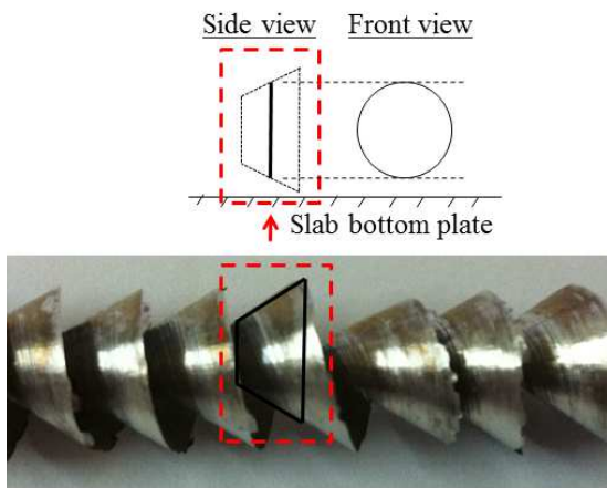
Fig. 4 Simplified computational model for spiral fillers
