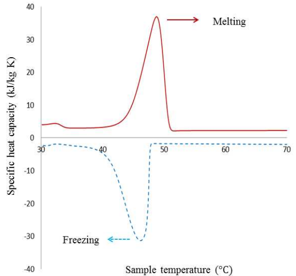
Fig. 2 DSC results for paraffin wax
