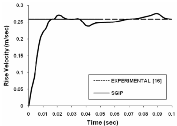
Fig. 6 Bubble velocity versus time for D=3 mm
