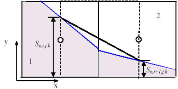
Fig. 2 Interface in a x- momentum cell and interface function S_x
