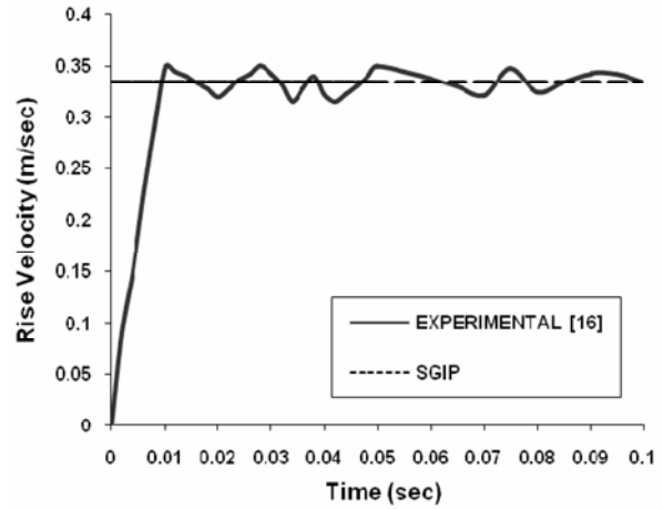
Fig. 5 Bubble velocity versus time for D=1.5 mm
