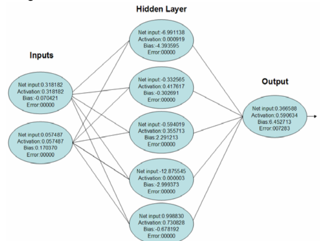
Fig. 2 The developed 2-5-1 feed-forward ANN
