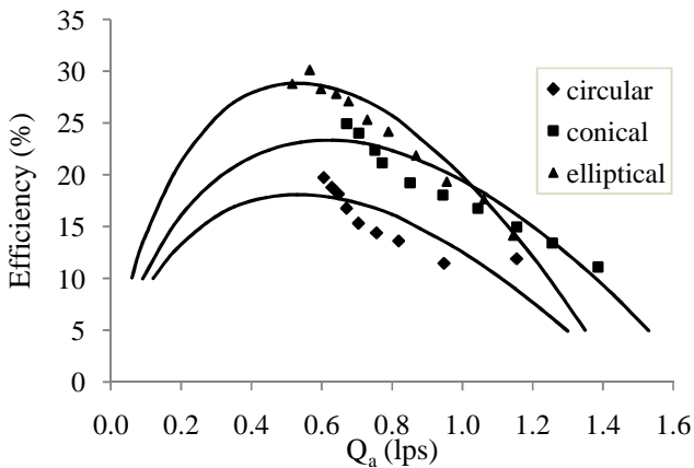
Fig. 8 Performance comparison at S = 32 mm & Q_w = 0.444 lps
