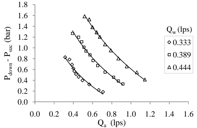
Fig. 5 Dimensional characteristic for elliptical profiled nozzle at 32 mm of nozzle spacing
