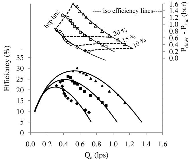
Fig. 9 Overall performance for elliptical profiled nozzle at 32 mm of nozzle spacing (legends are same as those on fig. 5 & fig. 7)
