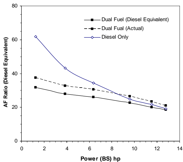
Fig. 7a. Variation of mass basis air-fuel ratio with increased diesel replacement by natural gas at different power levels.
