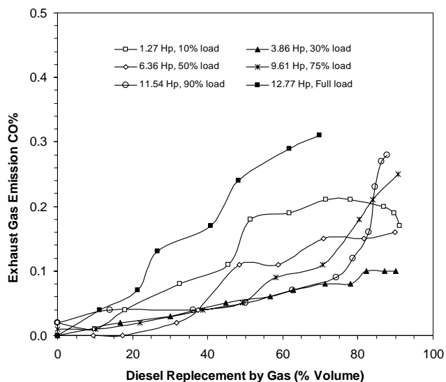
Fig. 10. Variation of CO 2 and CO emissions from diesel engine in Dual fuel mode.
