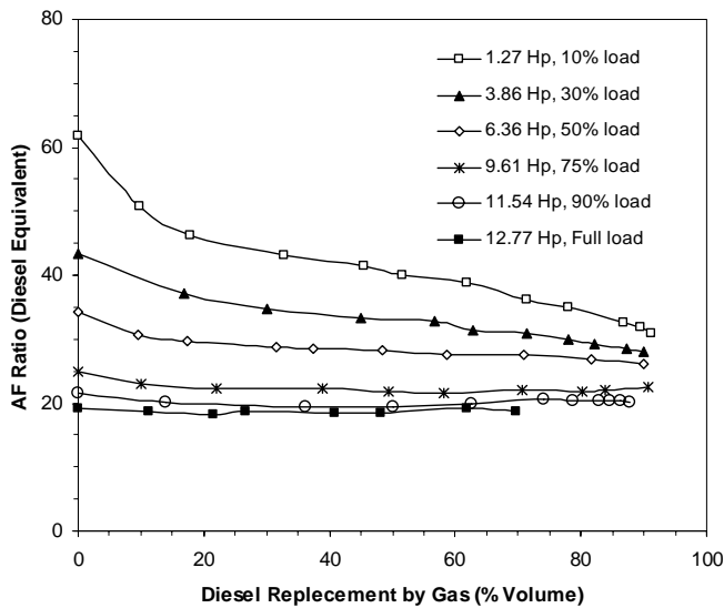
Fig. 7a. Variation of mass basis air-fuel ratio with increased diesel replacement by natural gas at different power levels.
