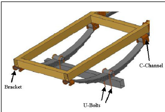
Fig. 2 : Arrangement of leaf spring in a car Model
