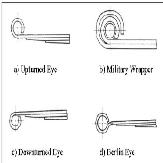
Fig. 4 : Types of Spring Eyes
