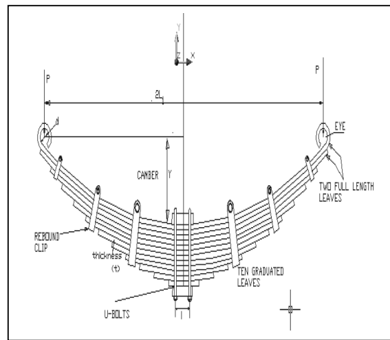
Fig.3 : Main Parts of Leaf Spring
