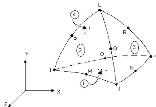
Fig. 5 : Solid 187 3D 10 node tetra hydral structure
