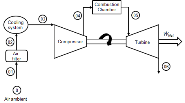
Fig. 2 Schematic of the gas turbine cycle with cooling system
