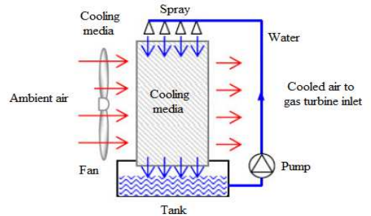
Fig. 3 Typical architecture of the evaporative cooling system
