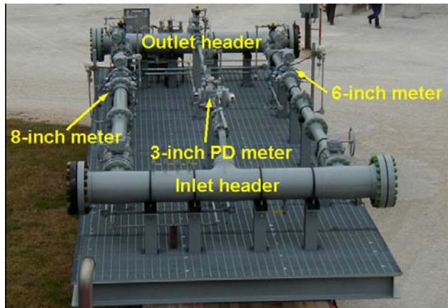
FIGURE 1. Power Plant Metering Skid Featuring Three Flow Meters in Parallel (i.e., one 8-inch diameter and one 6-inch diameter ultrasonic flow meter and one 3-inch diameter positive displacement (PD) rotary meter)
