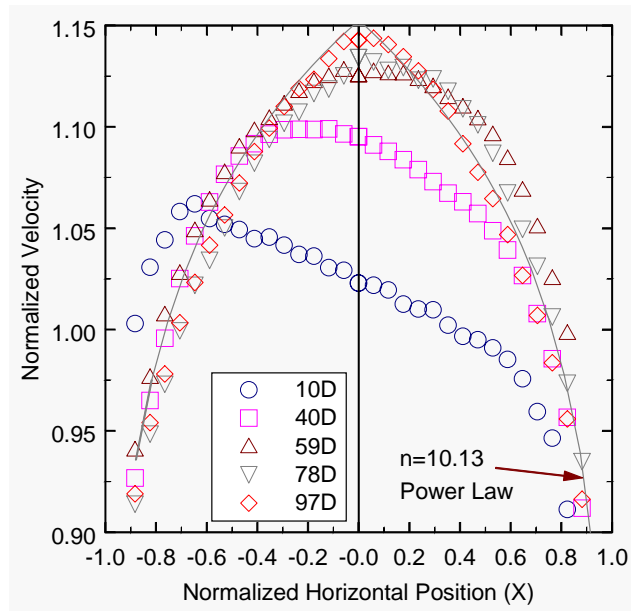
FIGURE 4. Centerline Velocity Profiles Measured Downstream of a Single, 90° Long-radius, Elbow [2]
