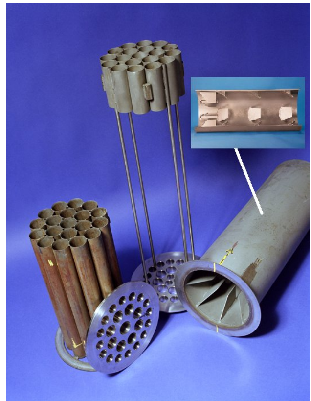
FIGURE 5. Example Flow Conditioners
