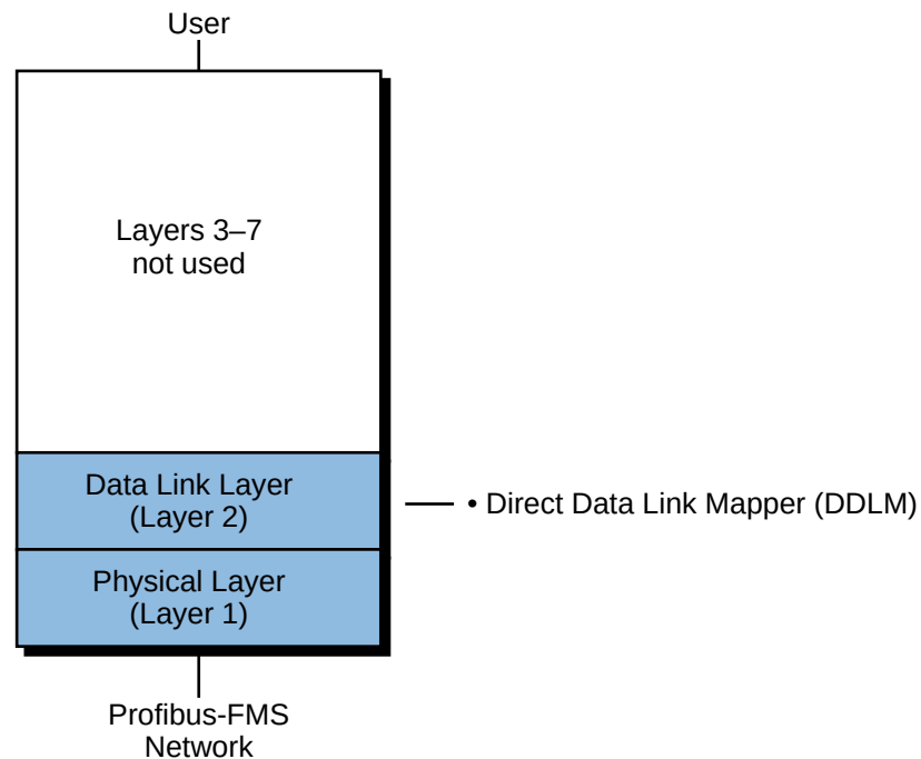
Figure 29. Profibus-DP protocol.
