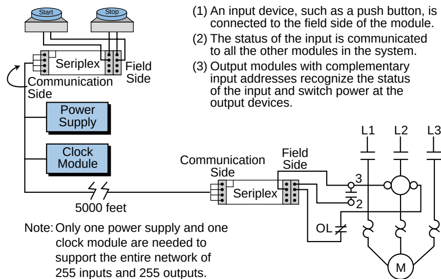
Figure 20. Seriplex I/O module interface without a controller.
