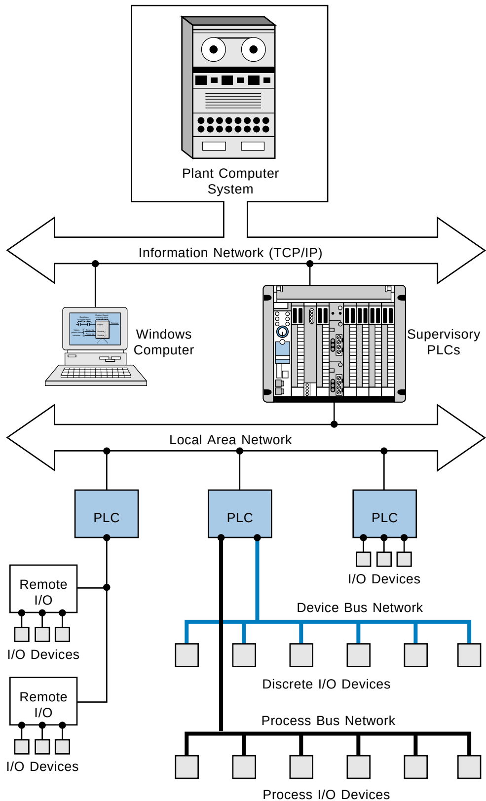
Figure 41. Large plantwide network.
