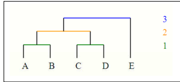
Fig. 5 : Two Cluster Examples
