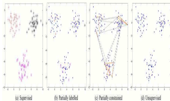
Fig. 1: Learning problems: dots correspond to points without any labels. Points with labels are denoted by plus signs, asterisks, and crosses. In (c), the must-link and cannot-link constraints are denoted by solid and dashed lines, respectively (figure taken from [Lange et al., 2005]).
