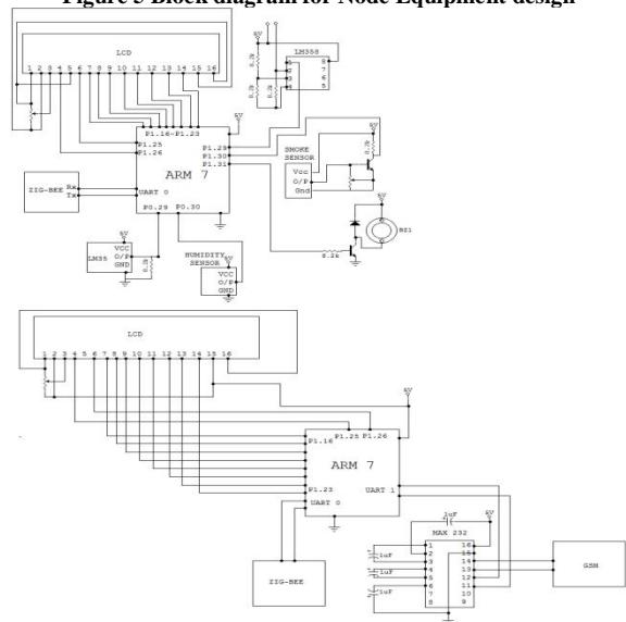
Figure 6 Circuit Implementation
