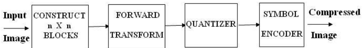
Fig 8.1: Block Diagram of Transform Coding System Encoder.
