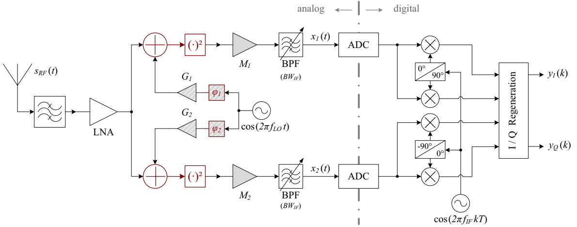
Fig. 1. Architecture of the Superposition Heterodyne Receiver with low analog complexity.
