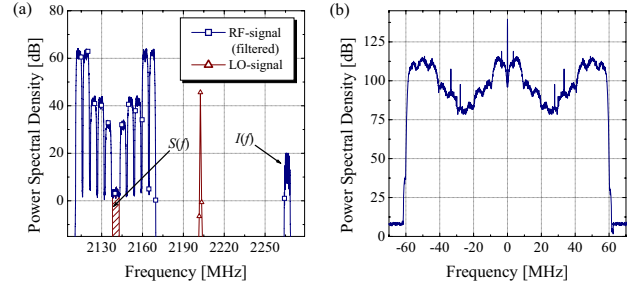
Fig. 3. Power spectral density of (a) the complete received RF-band, the image signal I(f) as well as the LO-signal at 62.5MHz offset apart from the desired channel S(f) and (b) the respective rectified wave.
