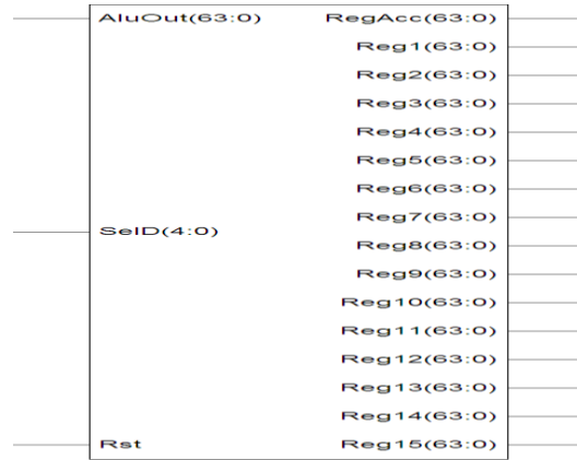
Fig.8: Block Diagram of GPR
