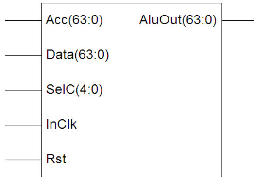
Fig.5. Block diagram of ALU
