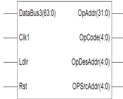
Fig.2: Block Diagram of Instruction Register
