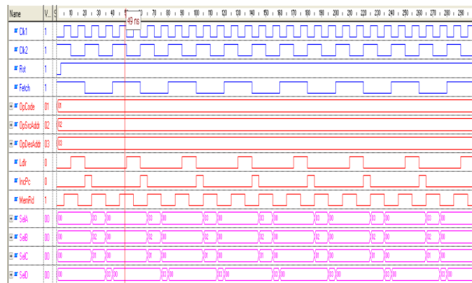
Fig.12: Simulation Results
