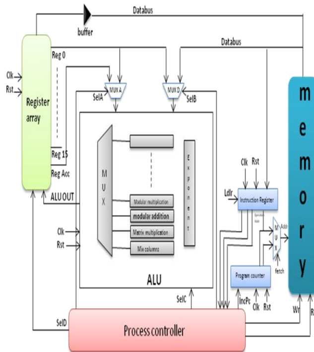
Fig.1: Processor Architecture
