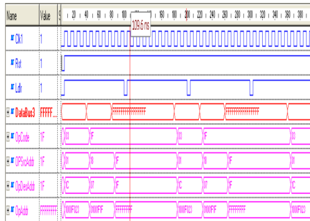
Fig.3: Simulation Results
