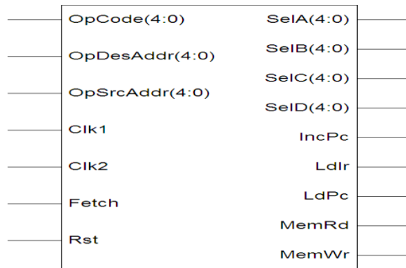
Fig.11: Block Diagram of Control unit
