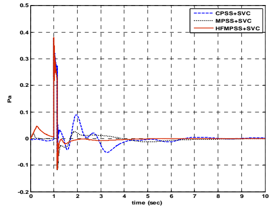
Fig. 20 Power deviation of machine 1
