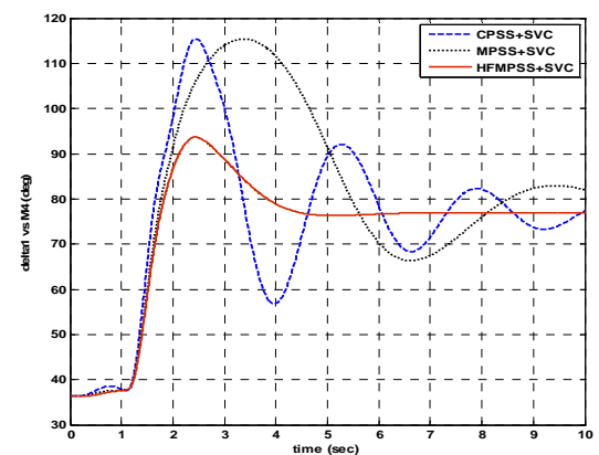
Fig. 15 Rotor angle deviation of machine 1 w.r.t. machine 4
