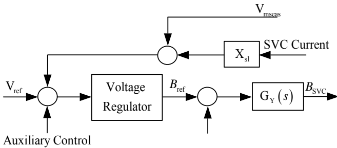
Fig. 6 SVC Controller
