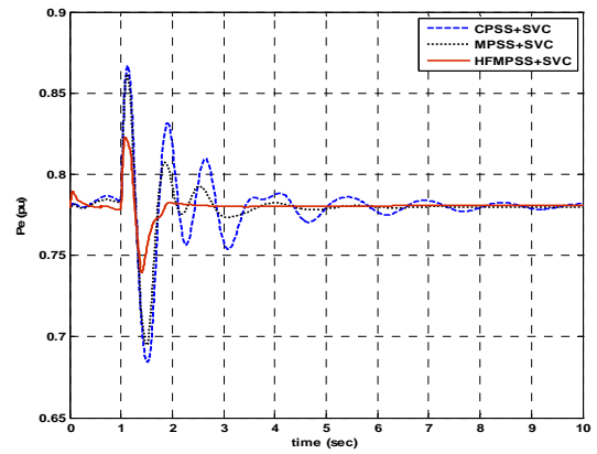
Fig. 14 Output power of machine 1
