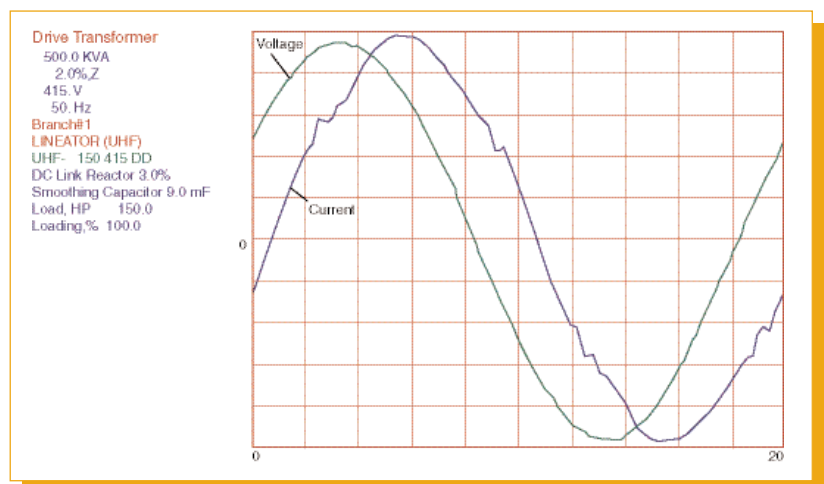
Figure 5. AC drive as illustrated in Figure 2 fitted with Lineator. I_{THD} = 5.1\% .
