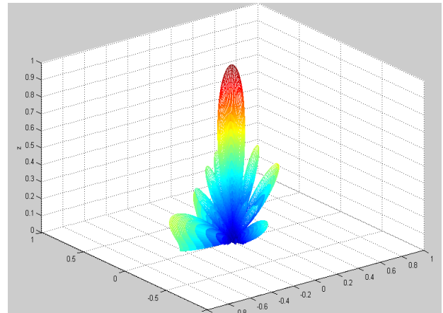
Fig 2. Uniform Distribution
