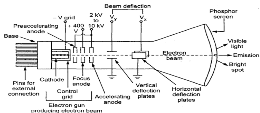
(fig) cathode ray tube
