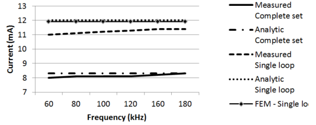
Fig. 2. Comparison of current values on the A_{10} loop for the complete antenna and single loop setups.
