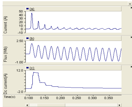
Fig. 3 : Transformer energization at switching angle 0° (a) Inrush current (b) Flux (c) DC component
