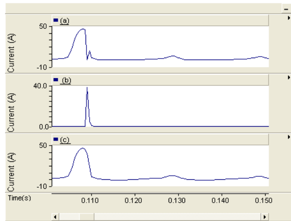
Fig. 6 : Current through a) GTO1 b) Pulse transformer c) Load transformer
