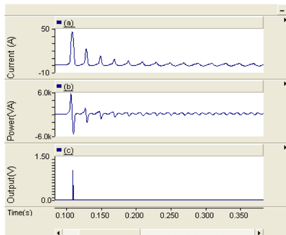
Fig. 4 : Transformer energization at switching angle 0° (a) Inrush current (b) Instantaneous power (c) Inrush current detection signal
