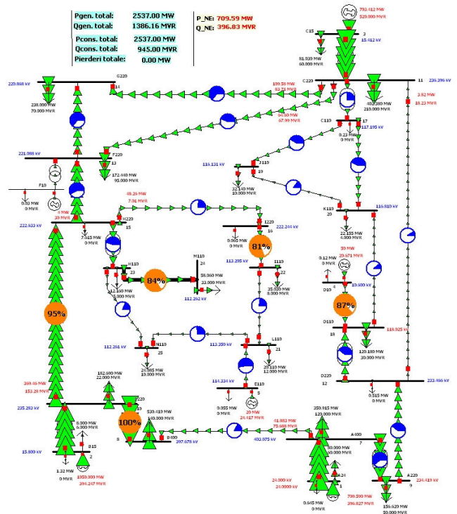
Fig. 3 Configuration of Test 25 buses test power system
