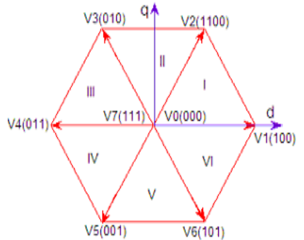
Fig. 2 Partition of the d-q planes in to six angular sectors
