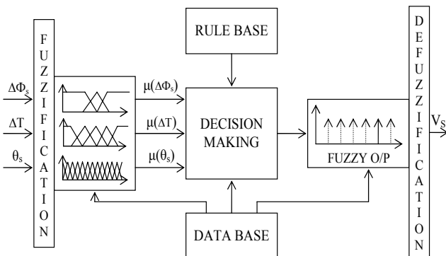
Fig. 3 Proposed DTFC functional block diagram
