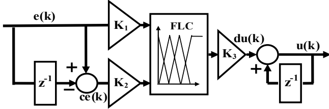
Fig. 5 Basic Structure PI-type Fuzzy Logic Controller
