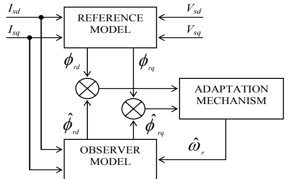
Fig. 6 Structure of MRAS Speed Estimator
