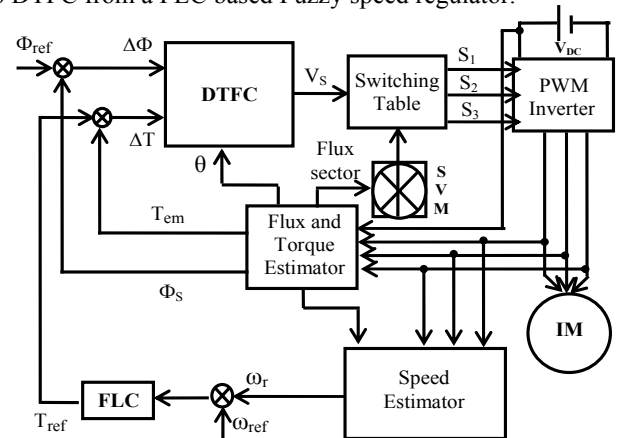
Fig. 1 Direct Torque Fuzzy Control scheme for AC motor drives with Fuzzy speed regulator
