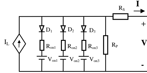
Fig. 5a Proposed PWL Model of PV cell
