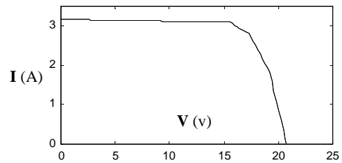
Fig. 6 I-V curve with the proposed model
