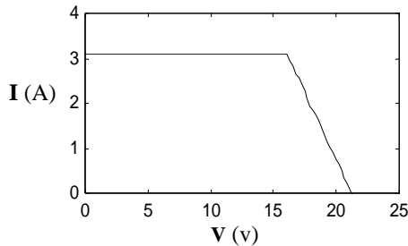
Fig. 10 I-V curve with classical model
