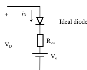
Fig. 2 Diode equivalent circuit used in Power System blockset/Simulink
