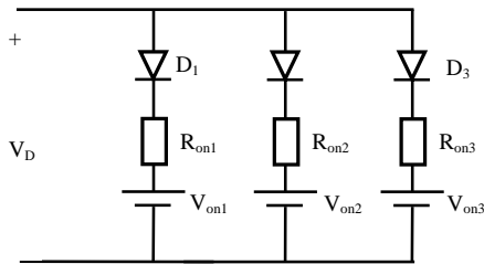
Fig. 4 Proposed PWL Model of PV diode
