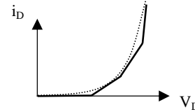
Fig. 5b Proposed diode model
