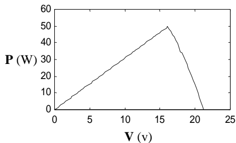
Fig. 11 P-V curve with classical model
