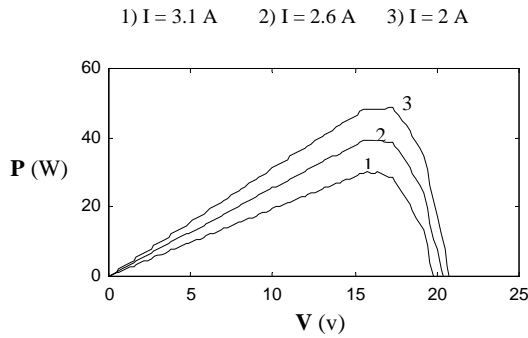
Fig. 9 P-V family curves with proposed model for different irradiation levels
