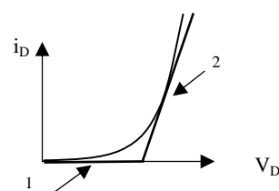
Fig. 3 Two-segment Diode model
