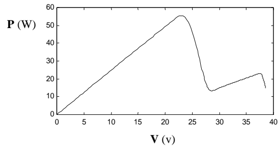
Fig. 12 P-V curve of simulated mismatched PV Panels
