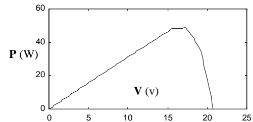
Fig. 7 P-V curve with the proposed model
