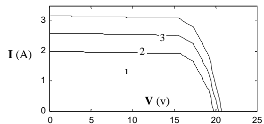
Fig. 8 I-V family curves with proposed model for different irradiation levels
