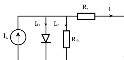
Fig. 1 Circuit model of PV solar cell
