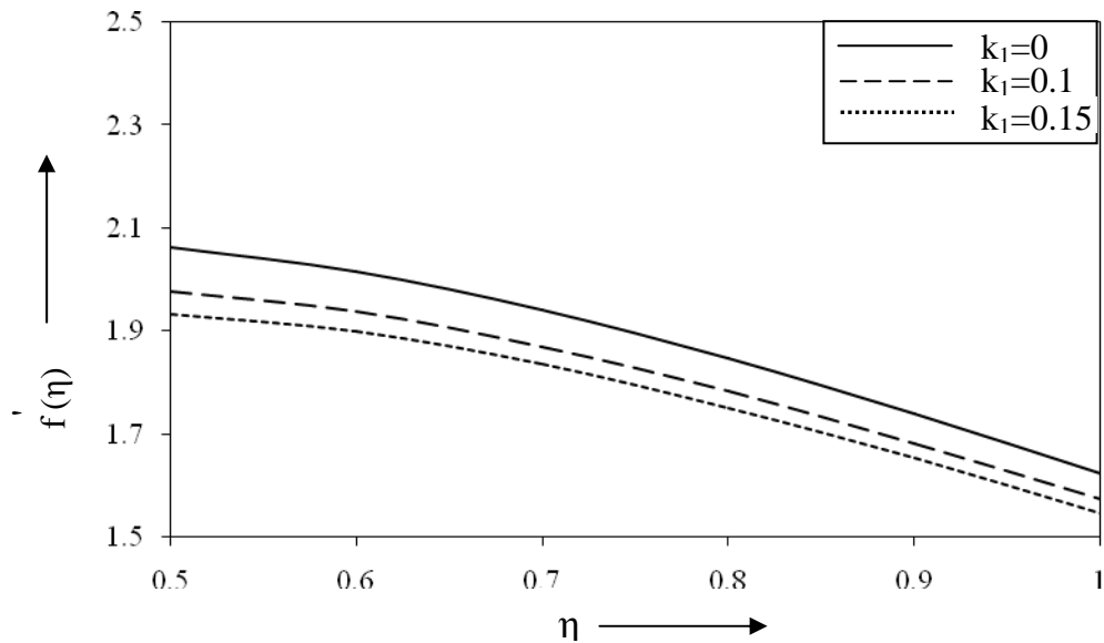
Figure 2: Velocity distribution against the variable \eta for M = 3
