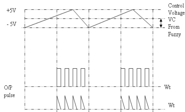
Fig.13. Generation of wave forms of TCA 785 IC
