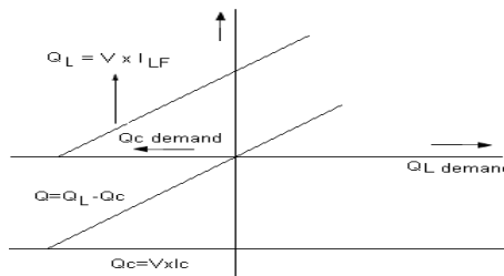
Fig.7. VAR demand versus VAR output characteristic
