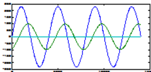
Fig.14. Uncompensated voltages for heavy loads
