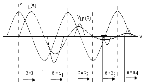
Fig. 3. Operating waveforms
