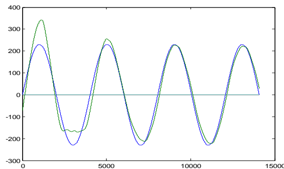
Fig.18. Compensated V_R = V_S (instantaneous voltage) For R=200 \Omega
