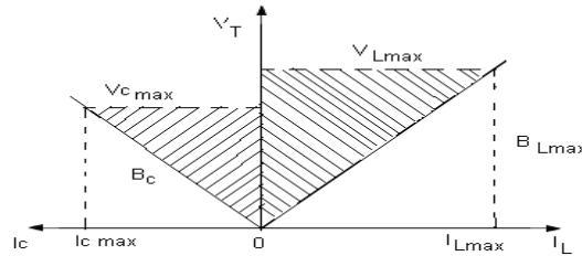
Fig.8. V-I characteristics of the FC-TCR type VAR Generator
