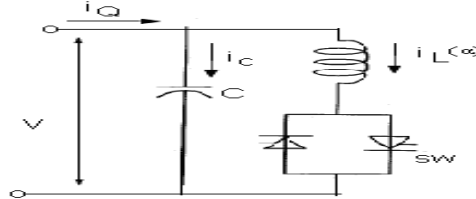
Fig.6. basic FC-TCR type static generator
