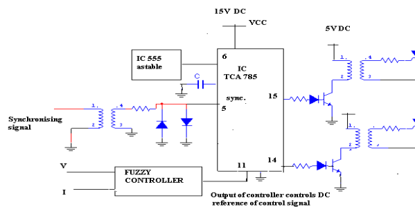
Fig.12. Firing Scheme with TCA 785 IC
