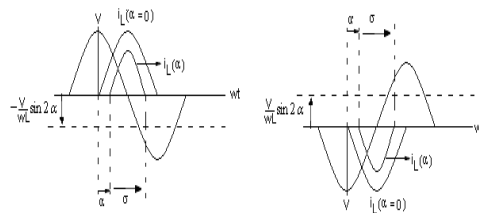
Fig.2. firing delay angle
