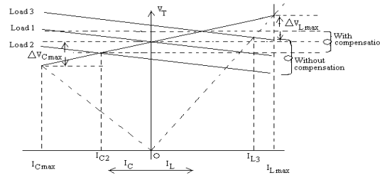
Fig.9. Dynamic V-I Characteristics of SVC with Load lines
