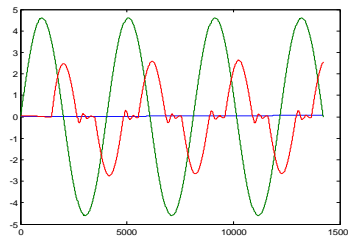
Fig.16. Inductor Current for firing angle 165 deg
