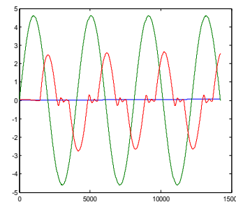
Fig.16. Inductor Current for firing angle 165 deg
