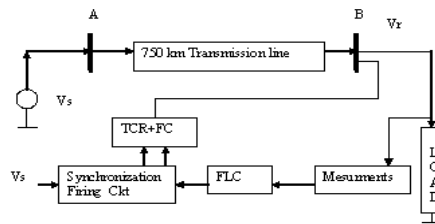
Fig.11. Single Phase equivalent circuit and fuzzy logic control structure of SVC
