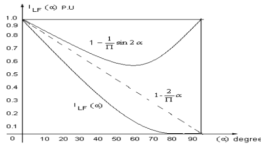
Fig.4. Amplitude variation of the fundamental TCR current with the delay angle ( \alpha )
