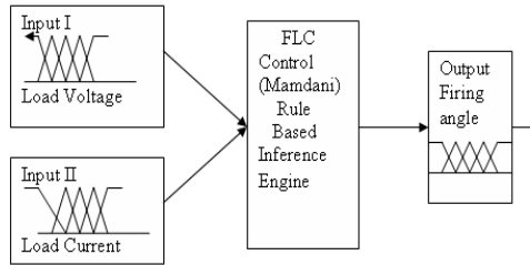
Fig.10. Structure of fuzzy logic controller
