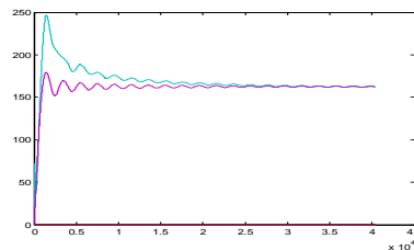
Fig.17. Compensated V_R = V_S (RMS voltage) for R=200\Omega
