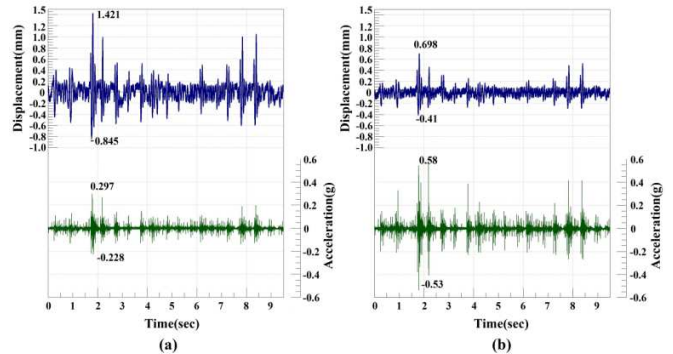
Fig. 8 Comparison of displacement and acceleration data for the insulator noise section: (a) new insulator; (b) used insulator generating noises
