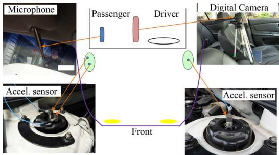
Fig. 2 Sensor installation position
