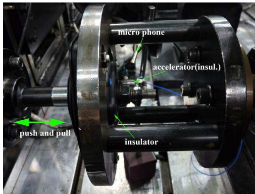
Fig. 11 Composition of insulator noise confirmation experiment devices
