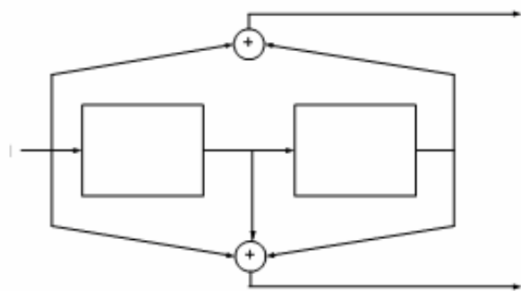
Fig. 5 Convolutional encoder r = 1/2, m = 2
