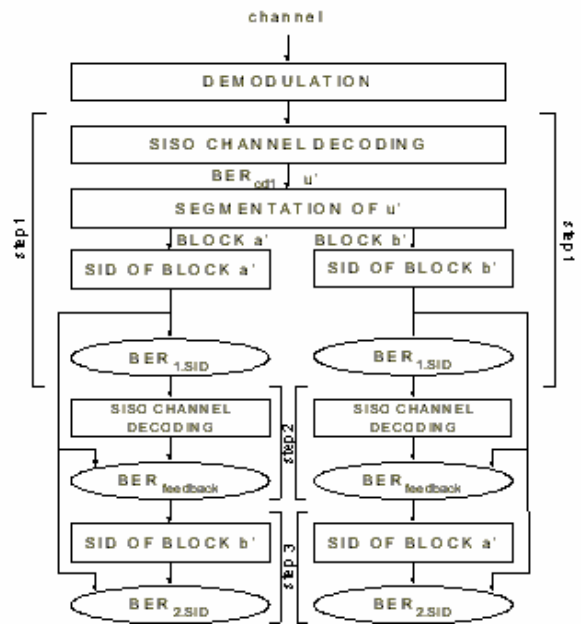
Fig. 4 Algorithm of Parallel Joint Channel Coding Cryptography
