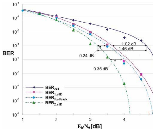
Fig. 6 BER after each step of Parallel Joint Channel Coding and Cryptography Algorithm, in comparison to 1/2 channel decoding
