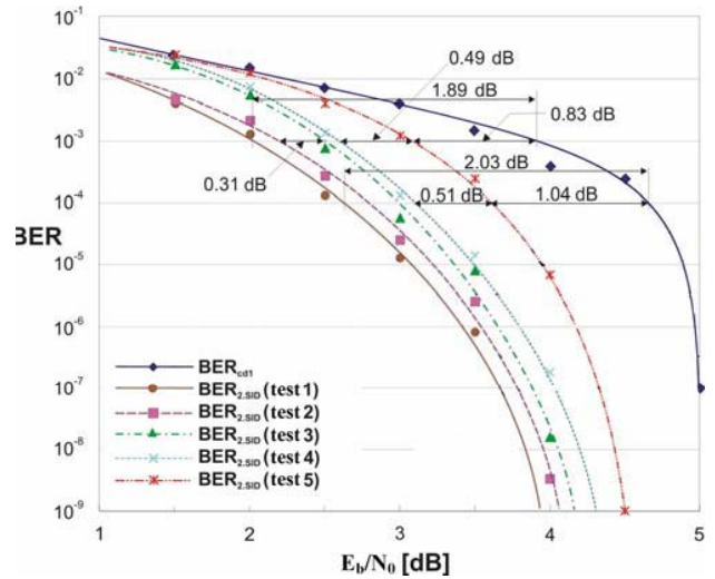
Fig. 7 Coding gains of Parallel Joint Channel Coding and Cryptography Algorithm of different block lengths, in comparison to 1/2 channel decoding
