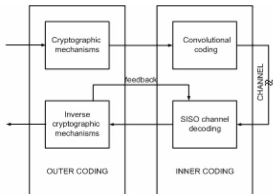
Fig. 1 Representation of channel coding and cryptographic mechanism as inner and outer code
