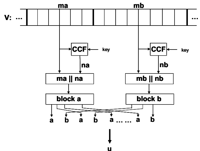
Fig. 3 Interleaving of blocks a and b into message u
