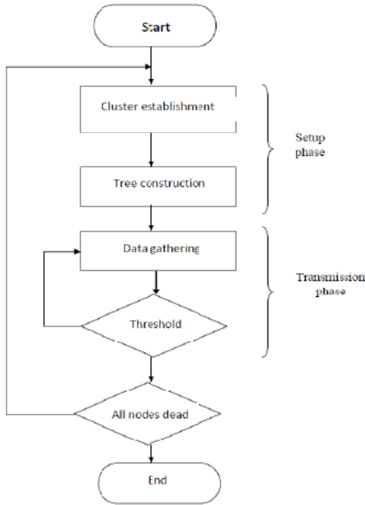
Figure 3 Flow chart of proposed protocol
